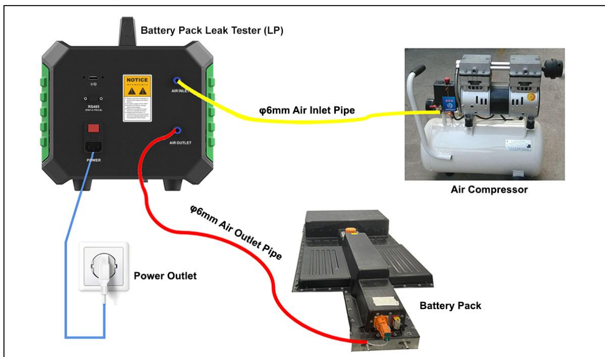
Connecting Diagram
