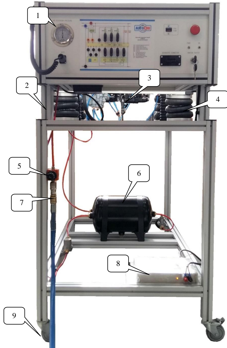
General view of the truck air suspension training stand
