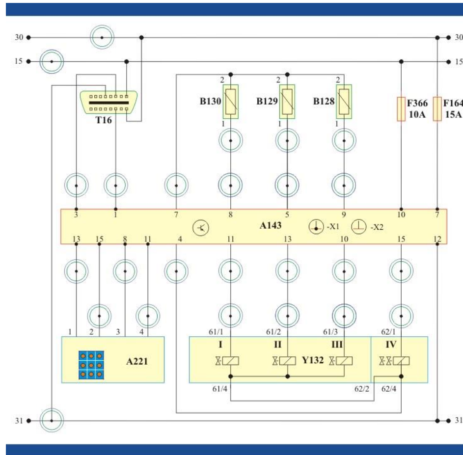
Wiring diagram of the truck air suspension system
